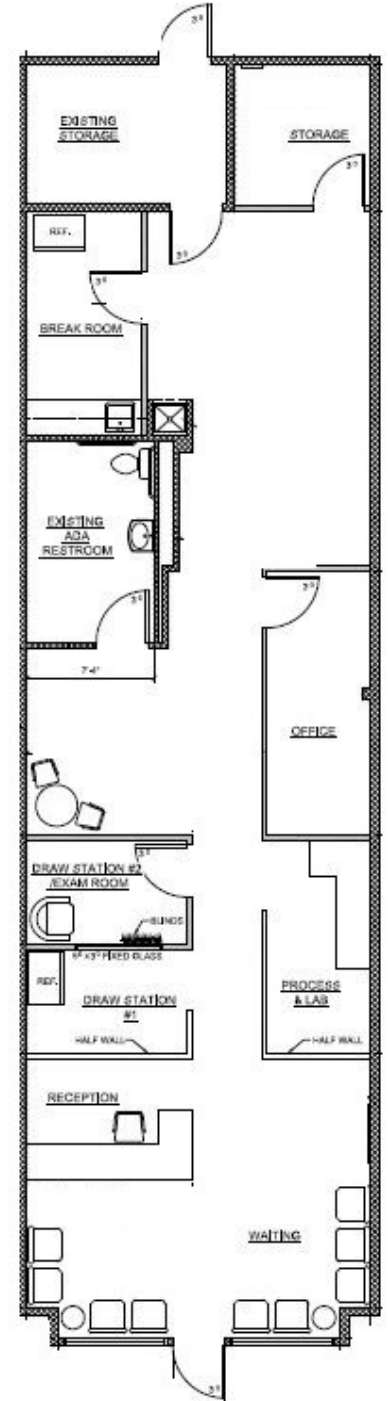
Floor Plan
